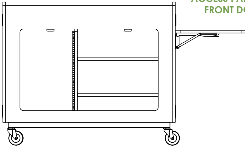
REAR VIEW
